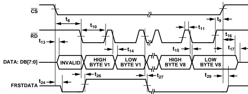
Figure 7. BYTE Mode Read Operation
