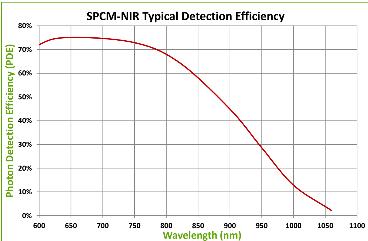
Figure 1. Typical Photon Detection Efficiency (PDE) vs. Wavelength
