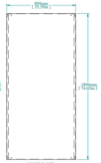
INNER PANEL
