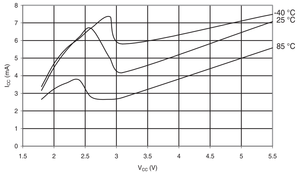
Figure 30-185. ATmega88PA: Programming Current vs. V_{CC}
