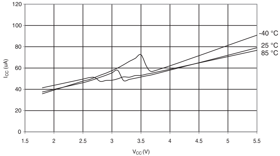
Figure 30-323. ATmega328: Analog Comparator Current vs. V_{CC}
