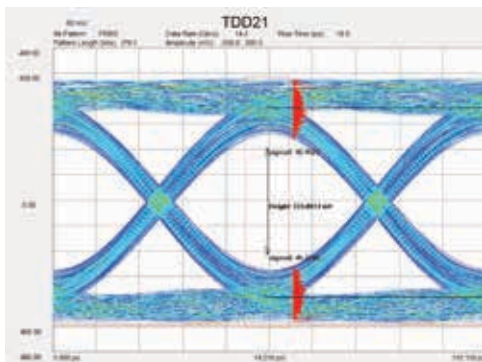
3M Cable 7700 Series 0.25m with 3M Socket, 451 Series and 3M SMT Header, 452 Series 14 Gbps Data Rate – 53% Eye Height
