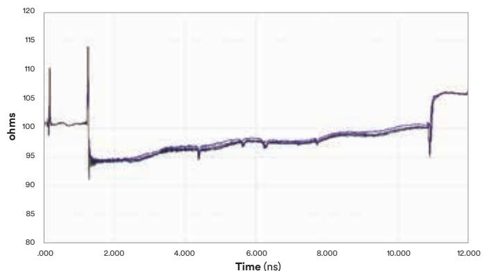
3M Cable 7700 Series Impedance Profile After 1008 hr 85° Heat Age with 5 Folds
