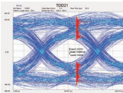
3M Cable 7700 Series 0.25m Cable Only 20 Gbps Data Rate – 73% Eye Height
