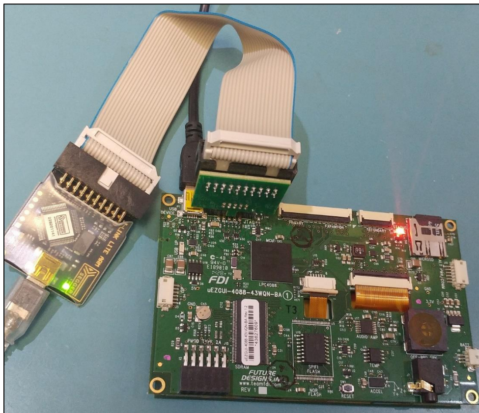
Figure 4: J-Link Connected to \mu EZ GUI
