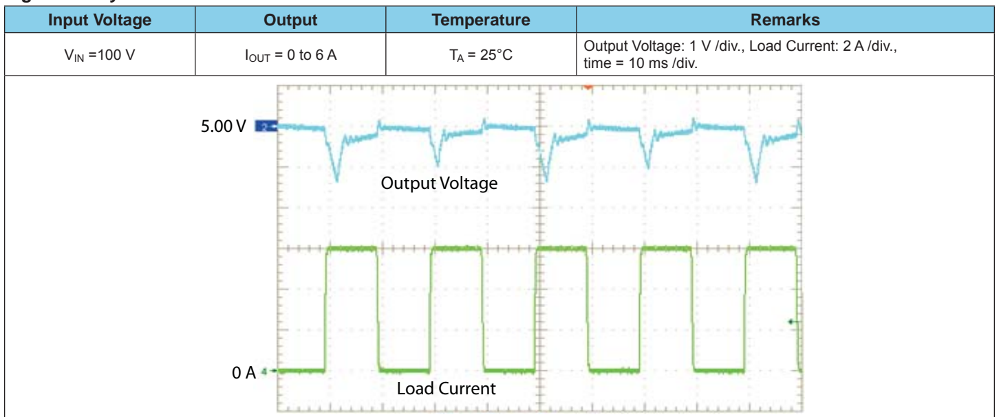
Figure 20. Dynamic Load
