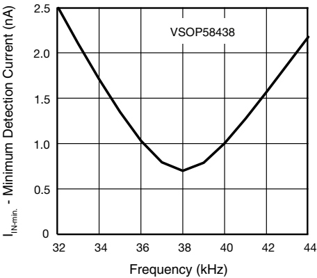
Fig. 4 - Bandpassfilter Characteristic
